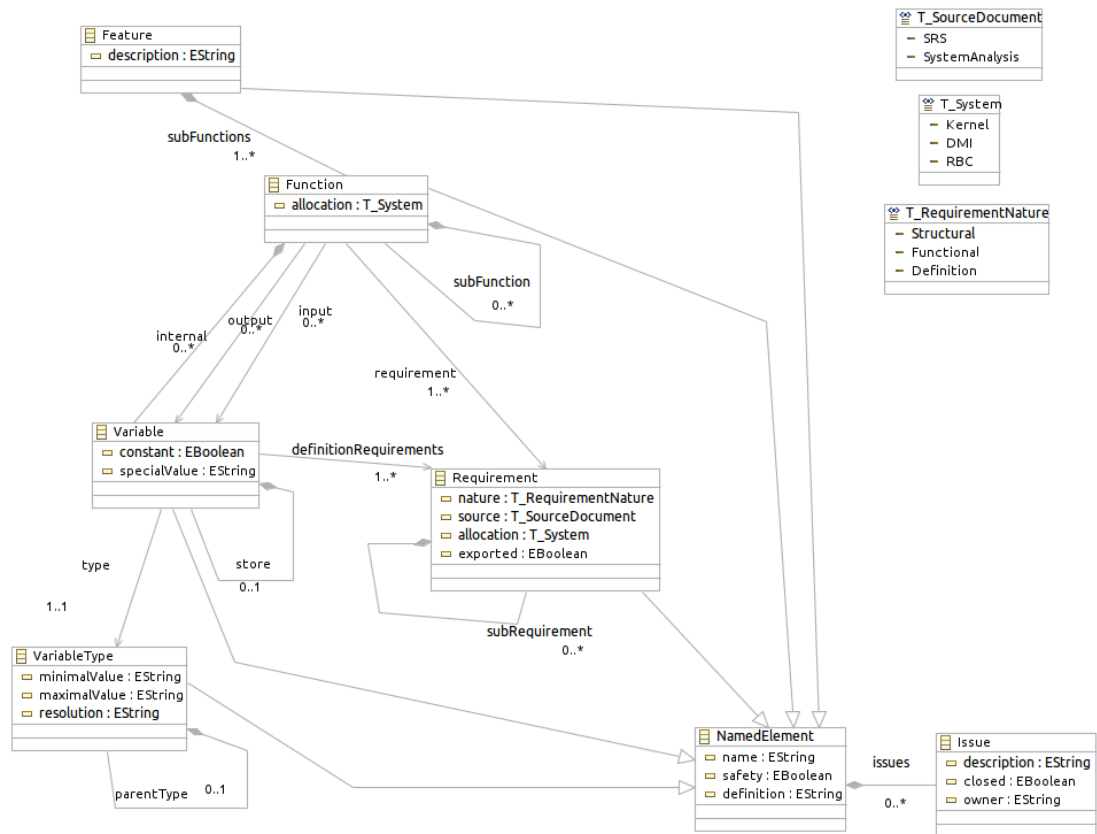
Figure 8. General Ecore model of the data dictionary
